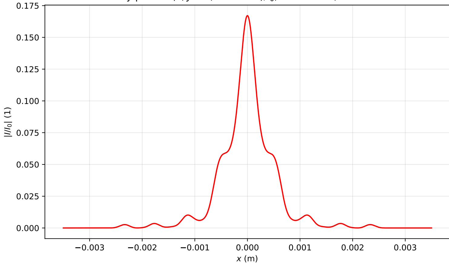
Intensity profile I(x, y = 0, z = 3.981)/I_0 , P_{in}=6.0P_{cr} , artificial time
